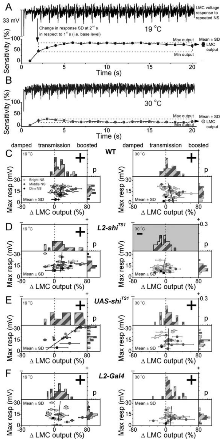
Figure 5. Genetic controls shows that adaptation in LMC output is dampened by reducing L2-R feedback. Statistical characterization of adaptive trends is for 4-days-old L2-shi TS1 , WT and control flies ( UAS-shi TS1 ; L2-Gal4 ), all having Canton-S (CS) red genetic association. The recordings are at 19°C (blue) and 30°C (orange). A. Typical high-quality voltage response of a LMC to a bright repetitive naturalistic stimulation (NS) at 19°C. This data is from a UAS-shi TS1 fly. Sensitivity, i.e. change in LMC output (gray circles) is defined as the mean of the standard deviations of consecutive response segments to a second long naturalistic stimulus (NS) pattern, from the 2 nd to 20 th s (dotted box, each data point is calculated from 800-ms data sections as in Fig. 2). This change is then plotted as a percentage, in respect to the 1 st response, showing 75% increase in the LMC output in 20 seconds. B. Voltage response of the same LMC, but at 30°C. Notice the faster adapting trend. LMC output increases 30% in 3 seconds before settling to 10%, due to faster bioreactions at the higher temperature [18]. Accordingly, the voltage responses at 30°C are often smaller than at 19°C. C–F. Changes in the mean LMC output of all recordings (with adequate stability) plotted against their maximum responses at 19°C (left) and at 30°C (right) for different flies as probability distributions. The left hemi-field indicates decaying and the right increasing LMC output. The fits show the mean correspondence between the adapting trends and maximum output. At 19°C, the fits lie to the right, i.e. the larger the response the larger is its adaptational boosting over the duration of the recording. C. WT Canton-S LMC output is boosted in 33/36 recordings (92%) at 19°C and 27/34 recordings (79%) at 30°C. D. L2-shi TS1 LMC output is boosted in 21/27 recordings (78%) at 19°C, but only 6/29 recordings (21%) show a small increase
