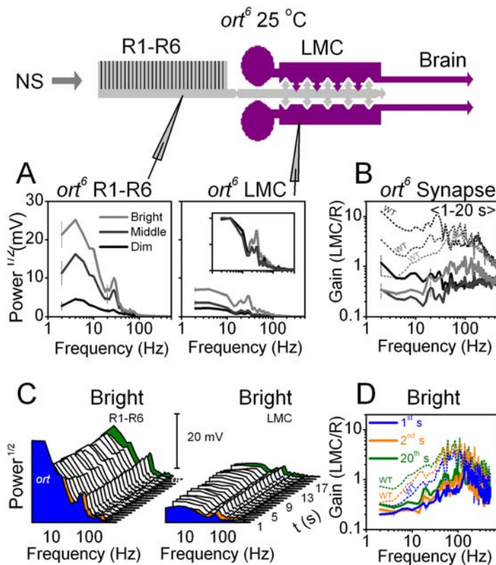
Figure 3. The ort 6 R-LMC-R system lacks adaptational enhancement of low frequency signals. A. Mean frequency spectra of seven ort 6 photoreceptors (left) and a representative LMC (right) to dim, middle and bright naturalistic stimuli (NS). Inset shows the normalized LMC frequency spectra. B. Synaptic gain is the highest with bright stimulation. Corresponding WT synaptic gain (dotted lines) is given for comparison, from [4]. C. Changes in ort 6 photoreceptor (left) and LMC (right) frequency spectra for 20 seconds of repeated bright stimulation. The 1 st (black), 2 nd (red) and 20 th (green) frequency spectra, respectively. D. The frequency range of ort 6 synaptic gain, dominated by high frequencies, spreads only marginally over time in comparison to the average WT Oregon-R synaptic gain (dotted lines) for the same experiment [4]. Error bars are SDs. doi:10.1371/journal.pone.0004306.g003
