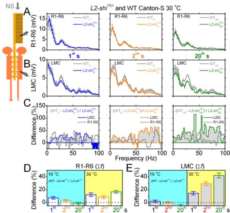
Figure 7. Adaptation acting through L2-R feedback helps to “whiten” LMC output. A. R1–R6 photoreceptor and B LMC mean frequency spectra for the 1 st (left), 2 nd (middle) and 20 th (right) voltage response of L2-shi TS1 (blue, orange, green) and WT Canton-S (gray) flies at 30°C. The recordings show mean ± SEM (photoreceptors: n = 7–9, LMCs: n = 5–12). C. The relative difference in the frequency spectra between WT and L2-shi TS1 LMC (gray areas) and photoreceptors (transparent areas under dotted lines). L2-R feedback “whitens” and extends the frequency range of LMCs over time by boosting mostly high-frequency signals (50–100 Hz). D–E. The panels show the mean ± SEM of the relative differences in C for R1–R6 and LMCs, respectively, at 19°C (white) and 30°C (gray). Gray bars differ significantly from white bars in all comparisons. L2-R feedback increases photoreceptor and LMC output by ~15% and ~40%, respectively, over time. doi:10.1371/journal.pone.0004306.g007
