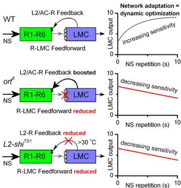
Figure 9. Feedforward and feedback pathways are necessary components for network adaptation. In the WT R-LMC-R system (top), LMC output increases with naturalistic stimulus (NS) repetitions by network adaptation (increasing sensitivity) set by a dynamic equilibrium between light-mediated conductance and feedback-mediated synaptic conductances. In the ort 6 R-LMC-R system (middle), mutated ort 6 histamine receptors act as a strict high-pass filter [8], reducing throughput of the feedforward pathway and depolarizing LMCs and AC. This amplifies the feedback connections to photoreceptors, pushing the dynamic equilibrium toward extreme “light adaptation” in all luminance levels. Thus, LMC output contains predominantly high-frequency signals and cannot be improved over time (decreasing sensitivity). In the L2-shi TS1 R-LMC-R system at 30°C (bottom), L2-R feedback is reduced and the dynamic equilibrium shifts toward dark adaptation. As less information is returning to photoreceptors, their output is modified less efficiently and the LMC output desensitizes, tracking mostly the photoreceptor adaptation (decreasing sensitivity). doi:10.1371/journal.pone.0004306.g009
