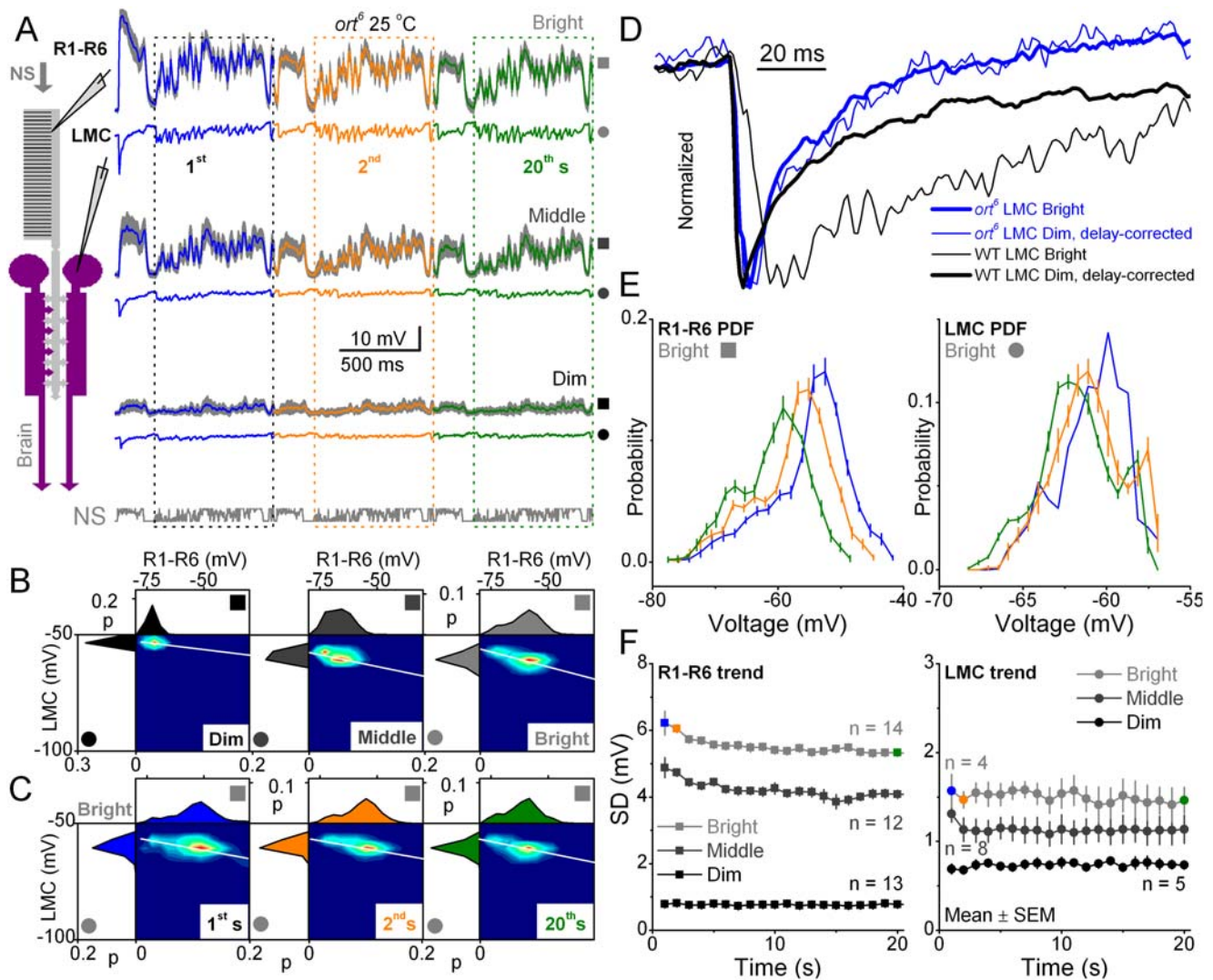
Figure 2. The ort 6 R-LMC-R system show limited adaptation to naturalistic stimuli (NS). Throughput of the feedforward pathway from R1–R6 photoreceptors to LMCs is compromised by ort 6 receptors, which reduce histamine sensitivity by >10-fold [8]. A. Voltage responses of ort 6 photoreceptors (mean \pm SD, gray, n = 7 ) and a representative LMC to a second long naturalistic stimulus (NS), during the first stimulus repetitions at different luminance levels at 25°C. B. The corresponding probability density functions (PDFs) for R1–R6s (top) and LMCs (left) and the joint probability density functions of the first 20 responses. In contour plots of jPDFs, hot colors denote high probability. The jPDFs quantify the input-output transformations, characterizing the synaptic gain for the given luminance of stimulation. The most probable synaptic gain, i.e. the slopes of the white lines, is quite invariable. C. The photoreceptor and LMC PDFs and jPDFs shown at the 1 st , 2 nd and 20 th s of bright stimulation. Note that the synaptic gain (white lines) varies little over time unlike in the WT system [4]. D. The normalized responses of ort 6 (blue) and WT Oregon-R LMCs (black) to dim (thin traces) and bright stimuli (thick traces). Ort 6 receptors mimic extreme “light adaptation”, making the speed (time course) of the LMC output invariable at different intensities. E. High resolution PDFs of photoreceptor (left) and LMC (right) outputs shown at different times during bright stimulation. The PDFs of ort 6 photoreceptors show a gradual compression in voltage range, whilst the PDFs of ort 6 LMCs remain unchanged after the first second of stimulation. F. The SDs of voltage responses indicate that the adaptive trends in the photoreceptor or LMC outputs are quite similar for each luminance level. Thus, sensitivity of these cells either remains the same or reduces gradually during repetitive stimulation, unlike in WT LMCs, in which the sensitivity increases over stimulation [4]. WT LMC output has an increasing trend, similar to Fig. 1C. SDs are from the boxed data (201–1000 ms) in A . doi:10.1371/journal.pone.0004306.g002
